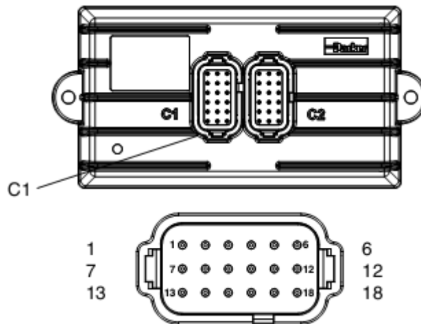
Figure 19: Connector C1
