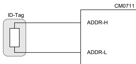
Figure 17: Module ID installation connections
