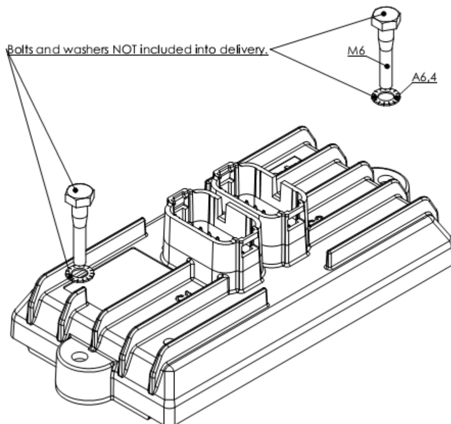
Figure 22: Mounting of the CM0711
