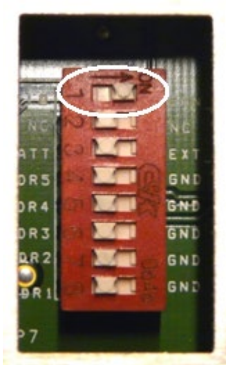
Figure 4: Recommended controller I/O board DIP switch configuration for the CM0711
