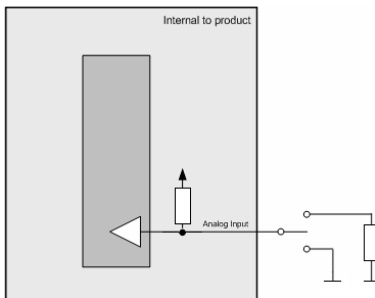
Figure 27: Connecting an analog input to an SPDT switch
